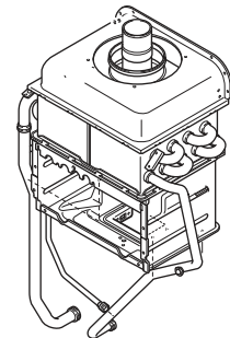
Heat Exchanger
